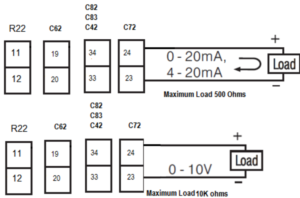
2-46. Retransmission Wiring
