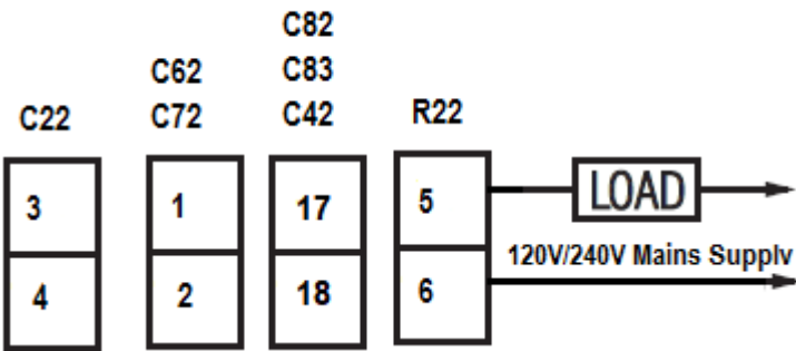
2-24. Output 1 Relay to Drive Load
