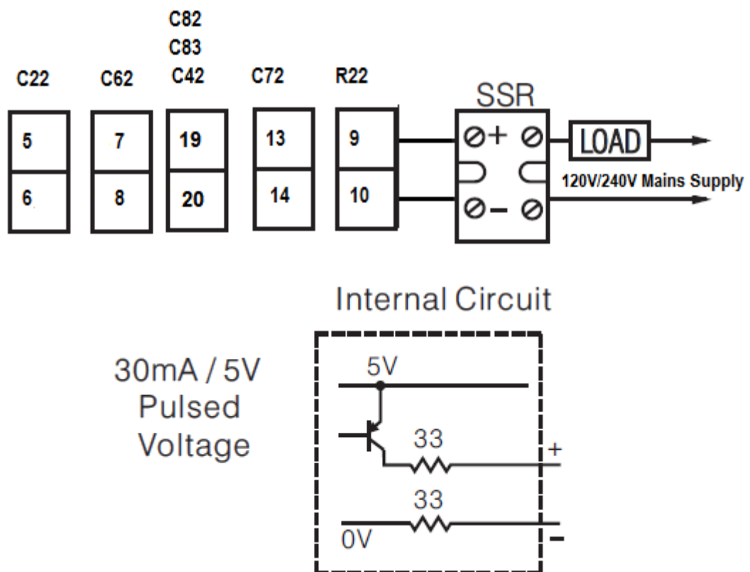
2-31. Output 2 Pulsed Voltage to Drive SSR
