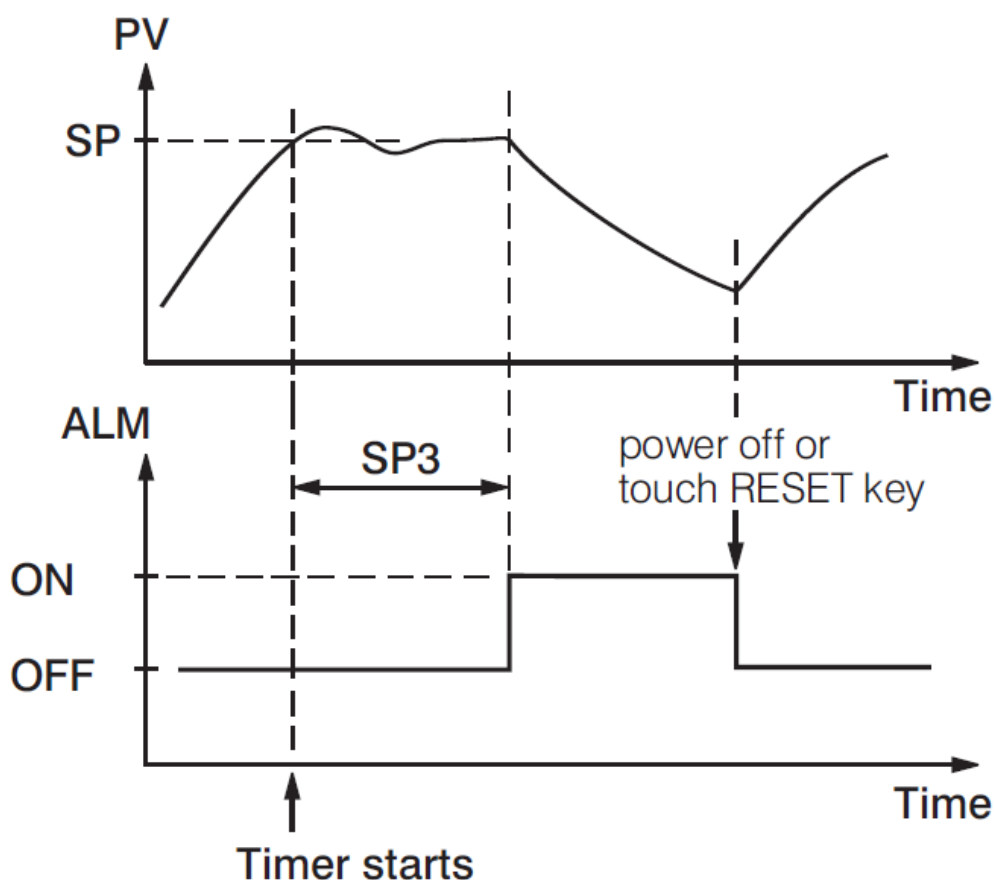
3-7.Dwell Timer
