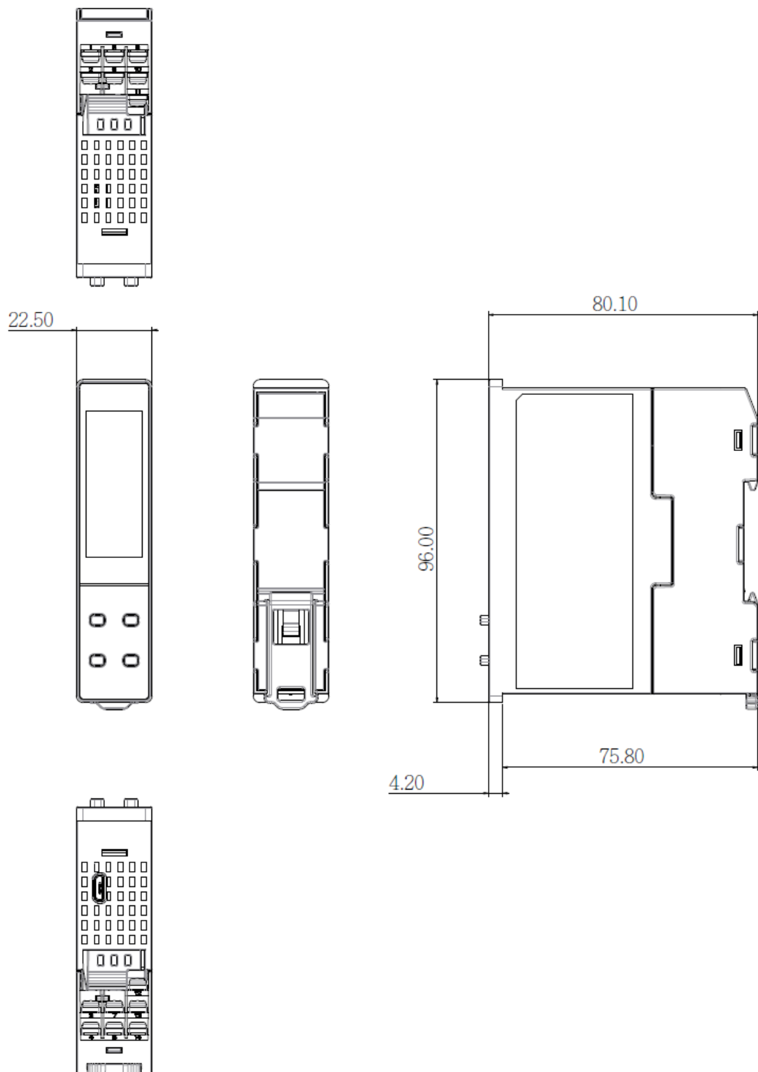
2-13.R22 Dimension
