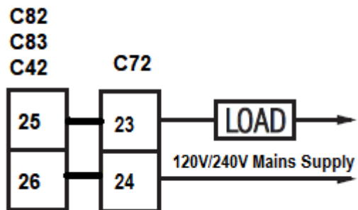
2-40. Alarm 4 Output to Drive Load
